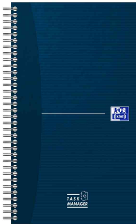
Task Manager
