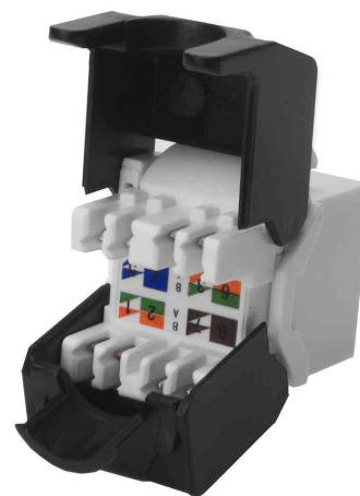
Keystone Modul Kat. 6, ungeschirmt, Details
