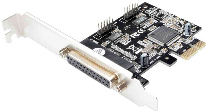
Seriell / Parallel MCS9901 SPP/EPP/ECP PCI-Express Karte, 2 seriell/1 parallel Port
